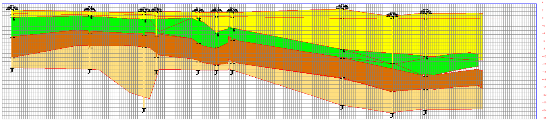
Alignment - 2 PROFILE
